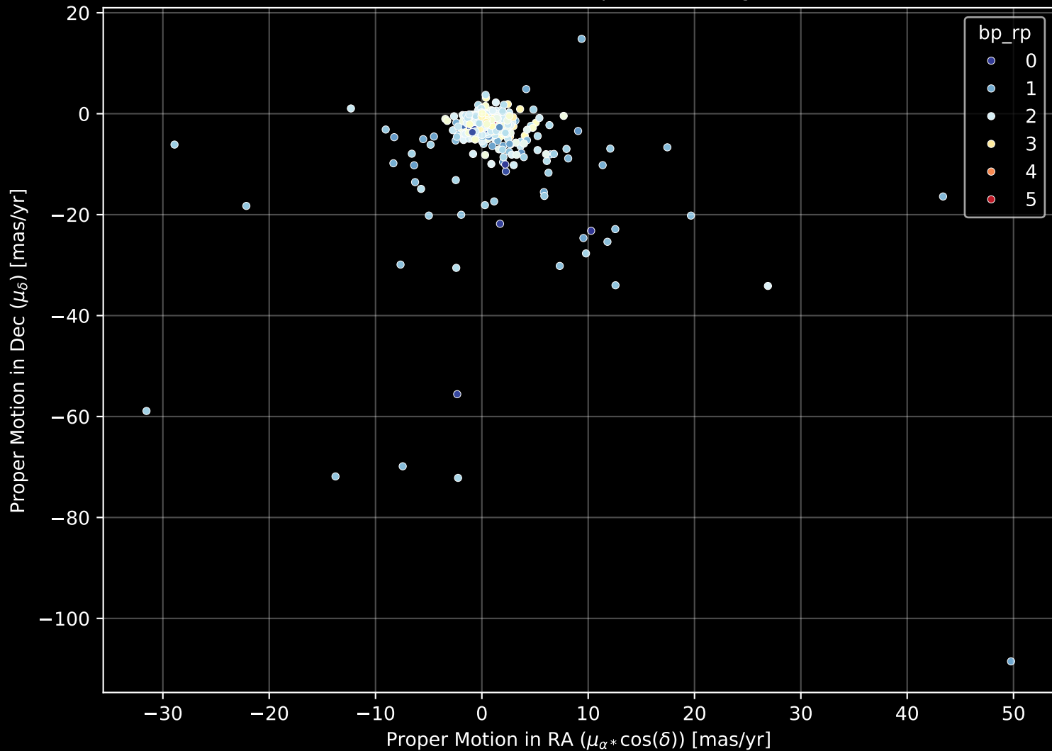
APOGEE DR17 Field: [176+00] Proper Motion Diagram (n= 498)
