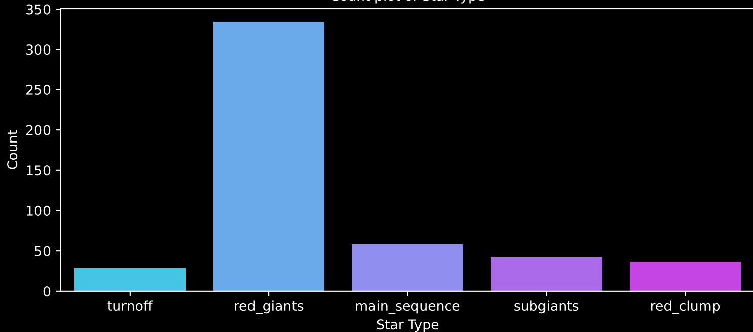
APOGEE DR17 Field: [176+00] Count plot of Star Type
