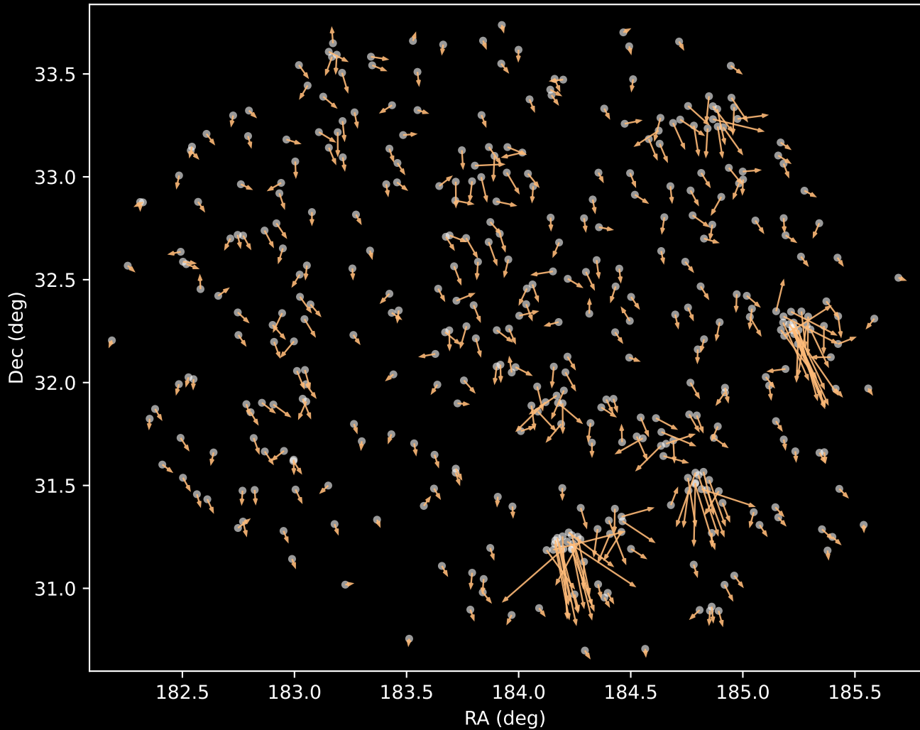
APOGEE DR17 Cluster 3 Proper Motion Vectors (n=398)
