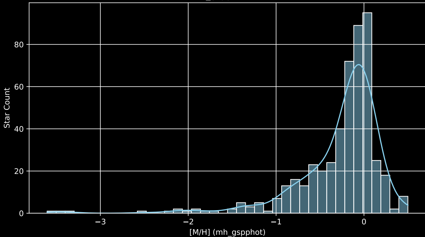
APOGEE DR17 Field: [176+00 [M/H] (mh_gspphot) (n= 493)
