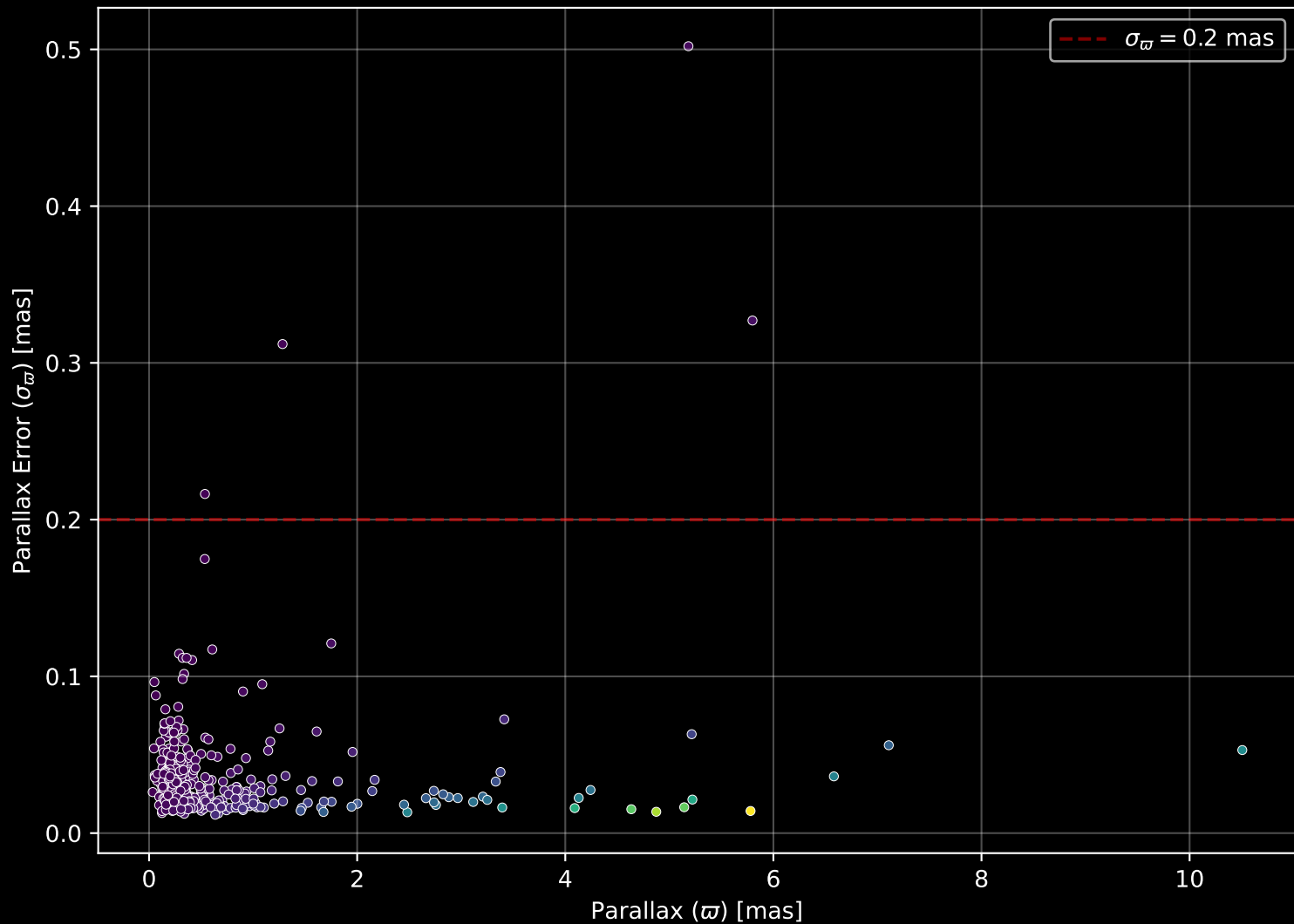
APOGEE DR17 Field: [176+00] Parallax Quality (n= 498)
