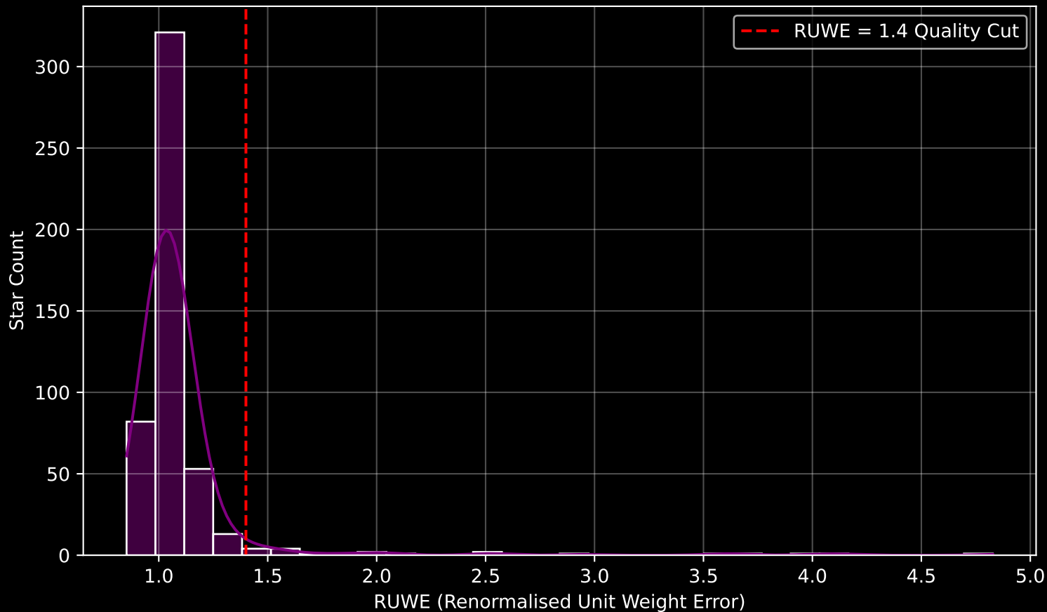
GAPOGEE DR17 Field [176+00] RUWE Distribution (n= 490)
